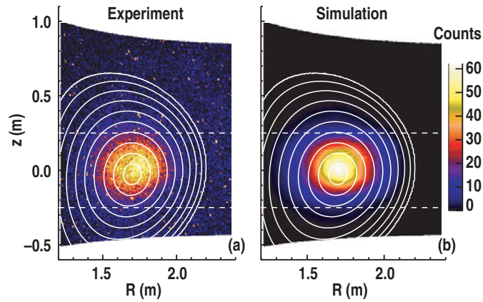
Figure 11. Experimental (a) and simulated (b) FIDA data from figure 8 plotted using R, z coordinates at which sightlines intersect the vertical plane defined by the 30L neutral beam injection vector. Overlaid \rho contours are calculated at the same R, z locations. Experimental data is the camera image at T2 minus that at T1 . Horizontal dashed lines indicate the 1/e extent of the neutral density plume.
