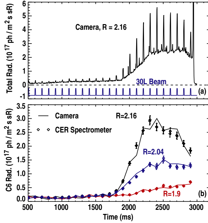
Figure 12. Discharge 135847 imaging data taken with C VI filter shown in figure 11, and camera frame rate of 300 frames s -1 . (a) Raw camera signal for pixel with beam intersection location (R, z) = (2.16, 0.0) m shown in black. Beam modulation waveform shown in blue. (b) Temporal evolution of active camera signal (obtained by removal of beam-off non-active signal) for three different midplane radial locations. Diamonds indicate CER spectrometer measured C VI brightness at same intersection locations. All camera data scaled by single constant to match CER data and obtain absolute calibration at 529 nm—same scaling constant was used to give absolute surface radiance values in panel (a).
