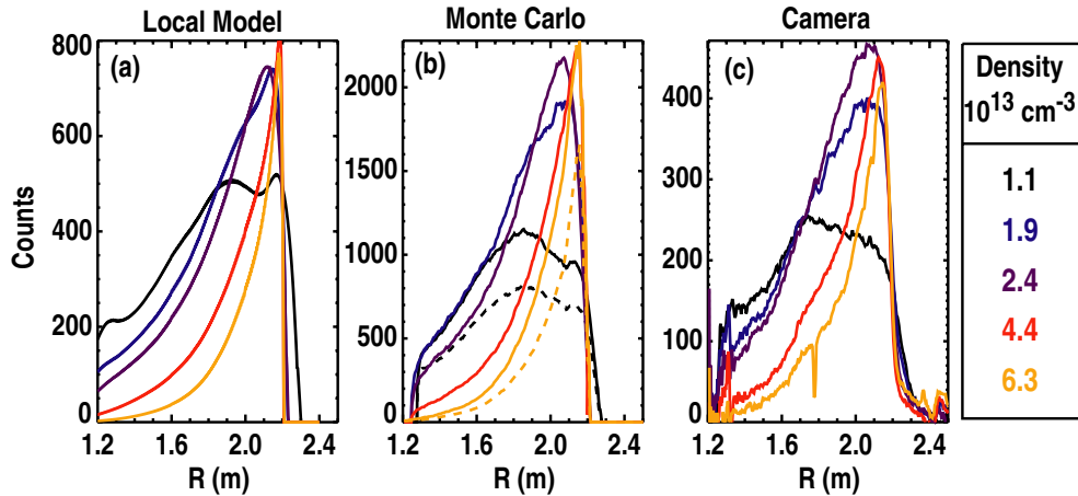
Figure 6. Modeling of midplane active D_\alpha camera measurements along the device midplane for the various density conditions shown in figures 4(a)–(e). (a) Results of local modeling using ADAS beam emissivity lookup tables and pencil beam neutral penetration calculations for the full, half and third energy neutral components based on experimental profiles of n_e , T_e and Z_{\text{eff}} . (b) Full Monte Carlo collisional radiative modeling calculations which include both beam emission and thermal deuteron charge exchange emission (solid). Dashed curves represent beam emission only for n_e = 1.1 \times 10^{13} \text{ cm}^{-3} (black) and 6.3 \times 10^{13} \text{ cm}^{-3} (yellow). (c) Camera measurements of active D_\alpha signal with vignetting removed for comparison with (a) and (b).
