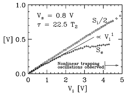
FIG. 9. The peak initial wave and echo wave wall signals, S_i and S_e , respectively, vs the initial wave excitation voltage V_i . The solid line is the theory prediction S_e \propto V_i .
