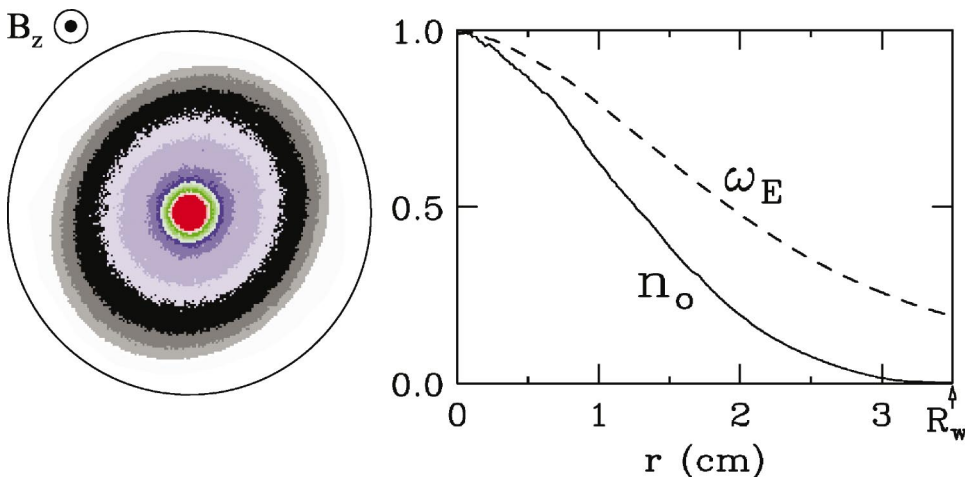
FIG. 3. (Color). CCD image of m=2 surface drift wave. Typical density n_o(r) and rotation frequency \omega_E(r) profiles are also shown.
