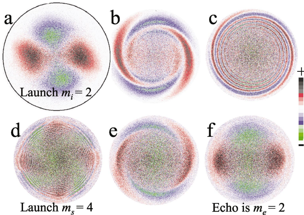
FIG. 5. (Color). Experimental density perturbation images at six successive times. The initial wave is excited in (a) and the density perturbation executes spiral wind-up as the wave is spatially Landau damped. (d) shows the second wave excitation and the echo peaks in (f).
