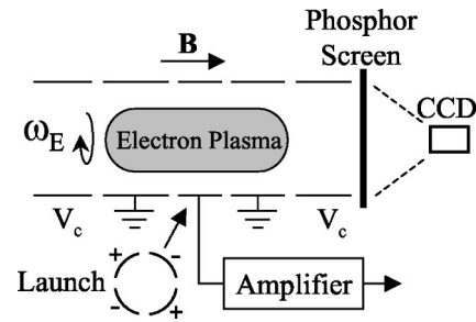
FIG. 2. Electron trap with CCD camera density diagnostic. The wall signal from sectored electrodes is used to measure the wave amplitudes.
