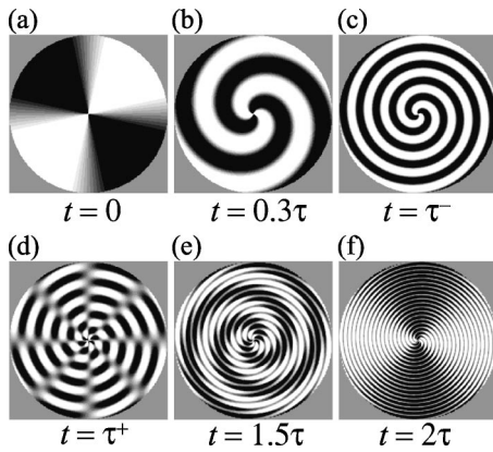
FIG. 1. Simple representation of phase mixing and unmixing, using (a) m_i = 2 and (d) m_s = 4 , resulting in (f) m_e = 2 .
