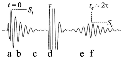
FIG. 4. Measured wall signal showing initial, second, and echo waves.
