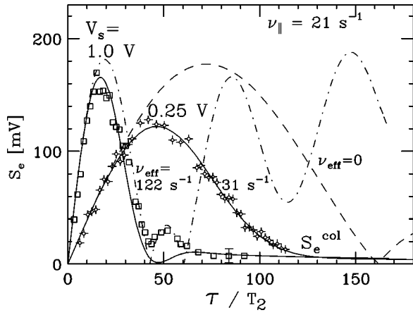
FIG. 7. Measured peak echo wall signal S_e vs the second wave launch time \tau for two different second excitation voltages V_s . The solid lines show fits from numerically integrating the collisional theory expression of Eq. (33). The dashed and dot-dashed lines have \nu_{\text{eff}}=0 .
