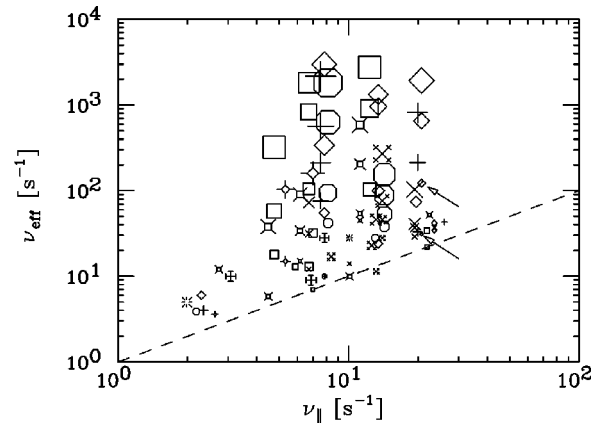
FIG. 8. Echo data showing the measured \nu_{\text{eff}} vs actual electron-electron collision rate \nu_{\parallel} . The size of the data symbols represents the strength of the second wave perturbation.
