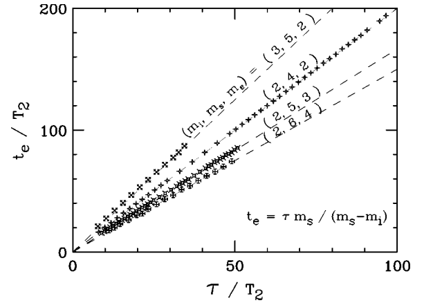
FIG. 6. Echo appearance time t_e vs the second wave launch time \tau , both normalized to the m=2 wave period T_2 , using various mode numbers.
