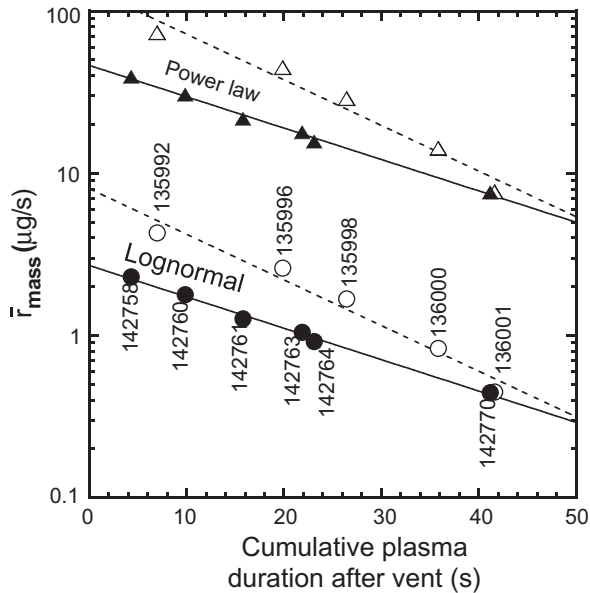
Fig. 4. Shot-averaged mass appearance rates \bar{r}_{\text{mass}} calculated for carbon dust after a vent with oxygen bake (solid data points) and after a vessel entry with no bake (open points), using both lognormal (circles) and power law (triangles) size distributions. The solid and dashed lines are exponential fits.
