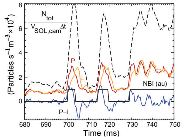
Fig. 2. Dust source ( P ) and sink ( L ) terms shown as the red and orange lines, respectively, with and without NBI (black solid line). P and L are calculated from total number of detected particles in each frame (black dashed line). Rate of change of dust density is shown as blue line. (For interpretation of the references to colour in this figure legend, the reader is referred to the web version of this article.)
